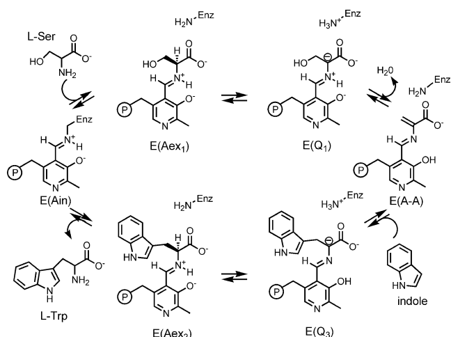
Scheme 1. An abridged catalytic cycle for the TS \beta -subunit reaction.
