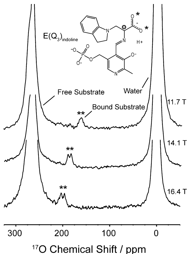
Figure 1. ^{17}\text{O} QCT NMR spectra of the E(Q_3)_{\text{indoline}} intermediate in TS at multiple magnetic fields. The enzyme-bound intermediates are marked with asterisks. Total number of transients and experiment times: at 11.7 T, 2.4 \times 10^6 transients and 22 hours; at 14.1 T, 2.2 \times 10^6 transients and 20 hours; at 16.4 T, 6.4 \times 10^6 transients and 59 hours. The spectra are displayed with 100 Hz line broadening applied. Experiments were conducted at 3 \pm 2^\circ\text{C} in pH 7.8 buffered aqueous solution. Additional experimental details are provided in the Supporting Information.
